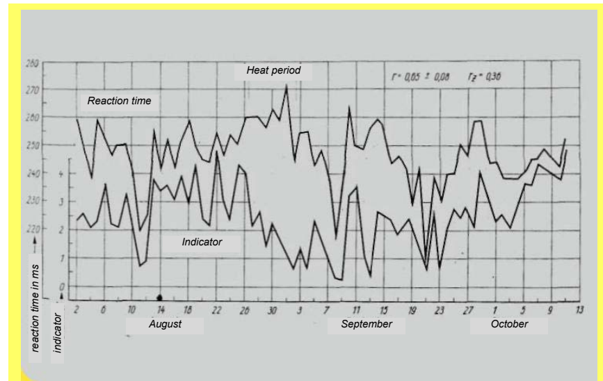
Fig. 5: Significant linear correlation between electromagnetic very long wave activity and average reaction times of exhibition visitors. Reiter, R. 1960 Meteorobiologie und Elektrizität der Atmosphäre. Akademische Verlagsges. Geest & Portig, Leipzig
